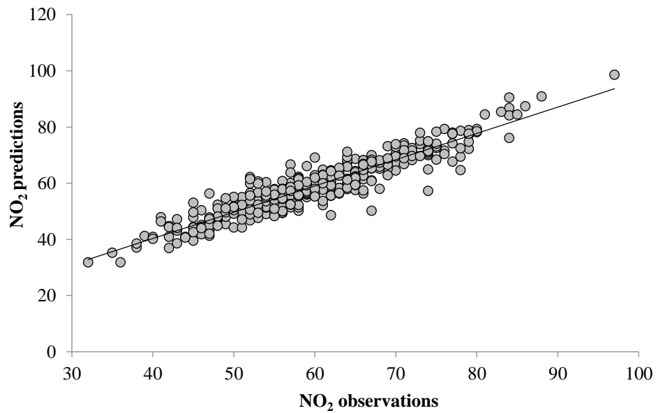
Figure 4: ANN predicted versus observation values for NO 2
